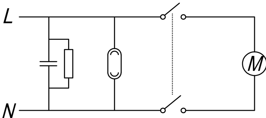
Schematic Diagram
